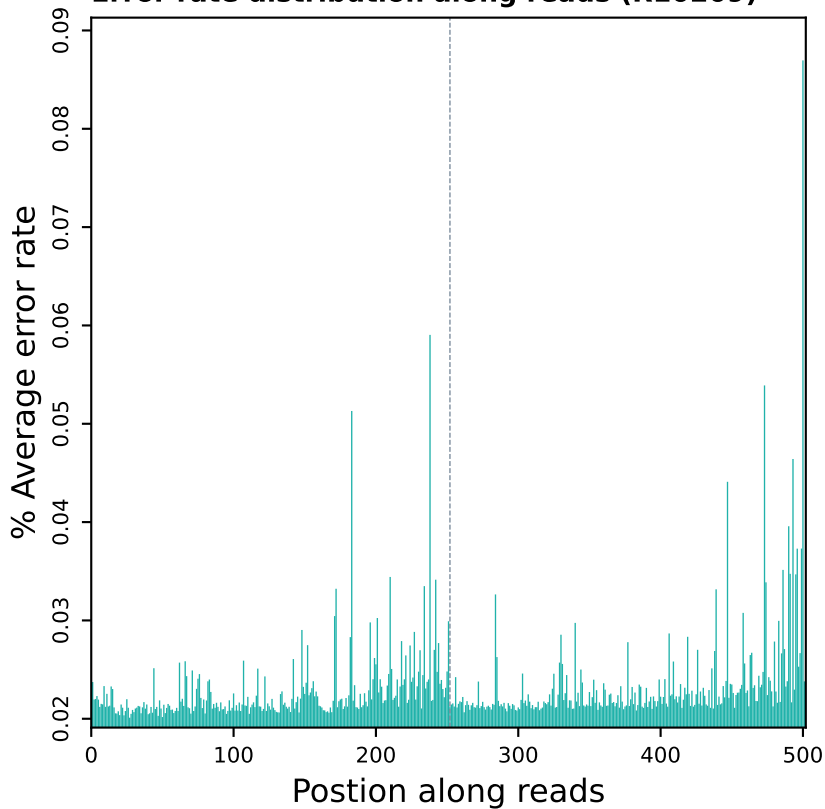
Error rate distribution along reads (R10209)
